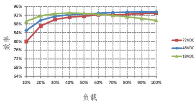
RSD-60H-5
