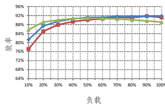
RSD-60H-12
