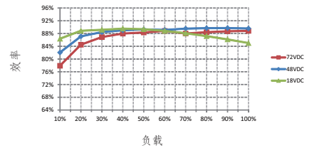
RSD-60H-3.3
