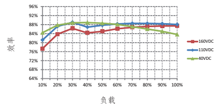
RSD-60H-24
